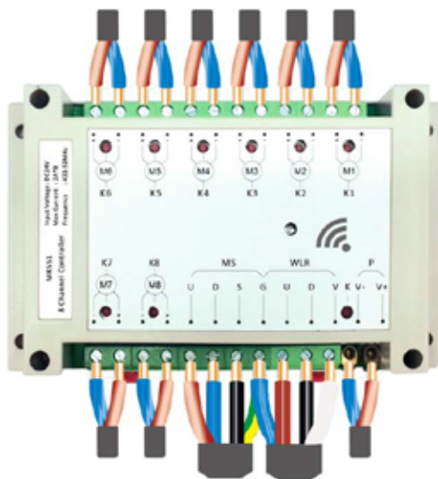
8 Channel Controller
