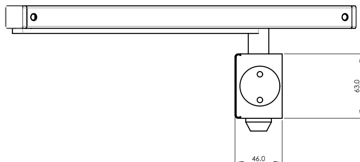
DC6001SA Door Closer with Slide Arm
