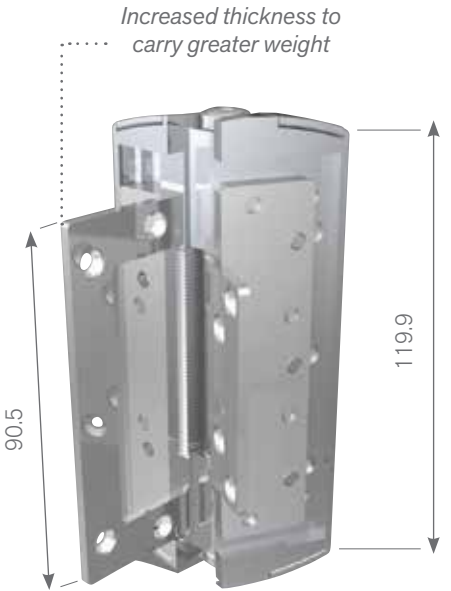
Bi-directional Fixing System
