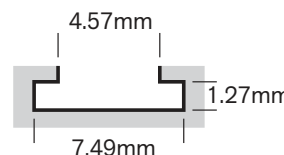
To suit 6.9mm Base Width
